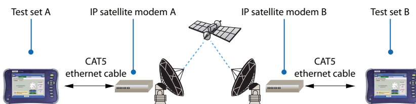
Figure 1. The T-BERD/MTS-6000A MSAM provides a full suite of testing features for turning up and troubleshooting satellite links
