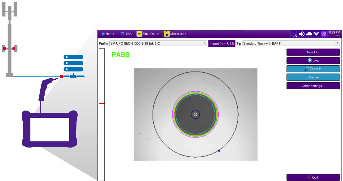
OneAdvisor-800 Fiber Inspection
