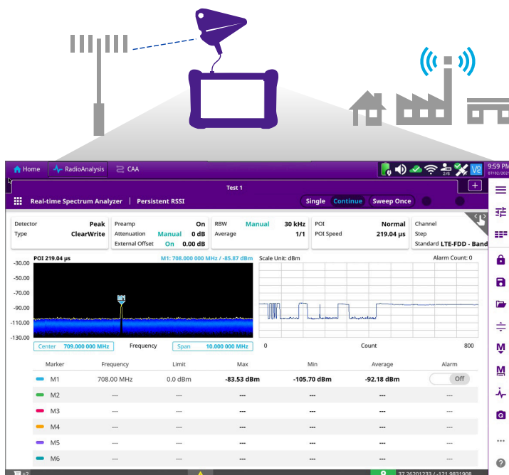
OneAdvisor-800 Interference Analysis (RSSI)
