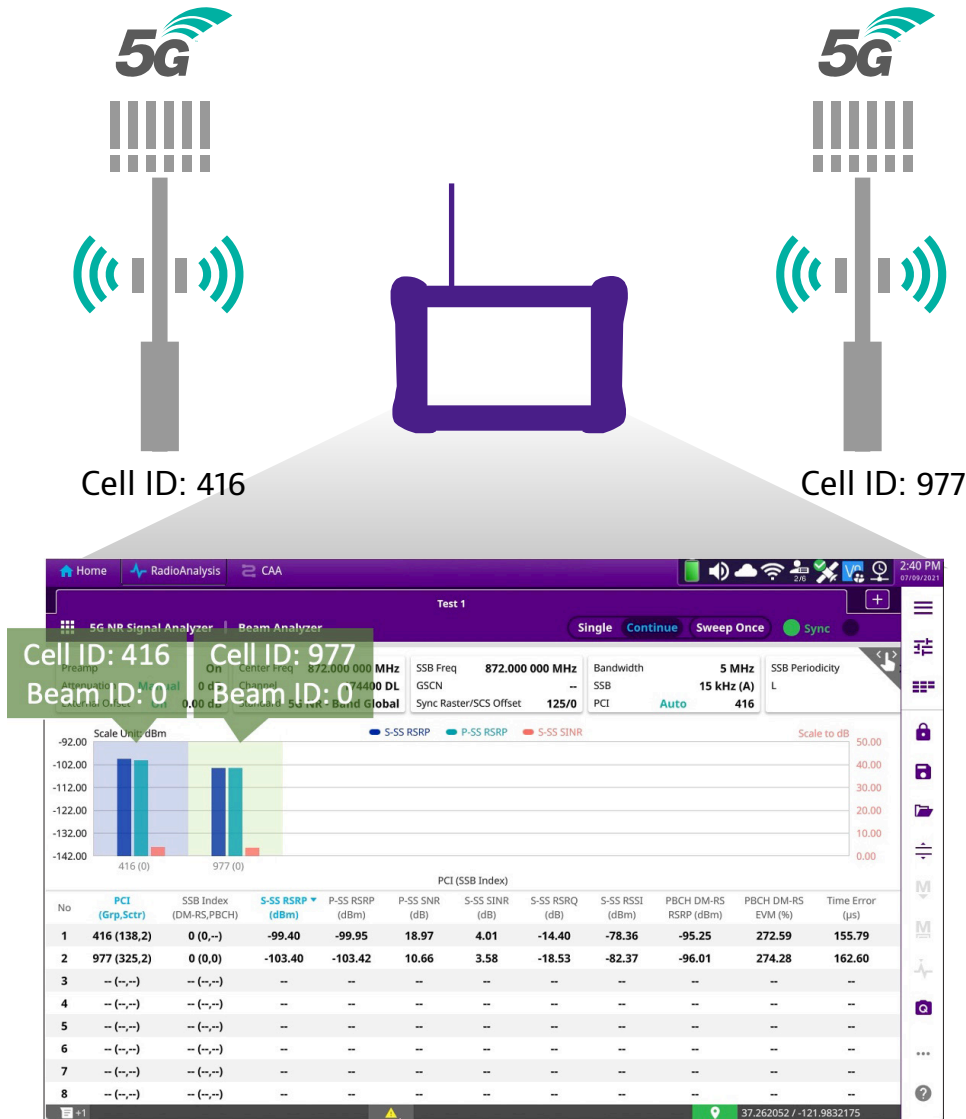
OneAdvisor-800 5G Signal Analysis – Beamforming
