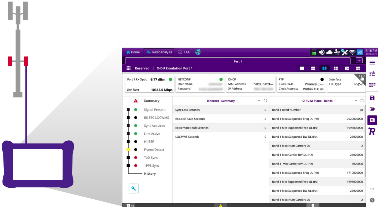
OneAdvisor-800 O-RAN ODU Emulation Verification
