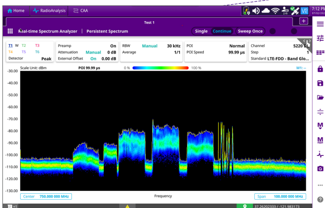
OneAdvisor-800 Real-time Spectrum Analysis
