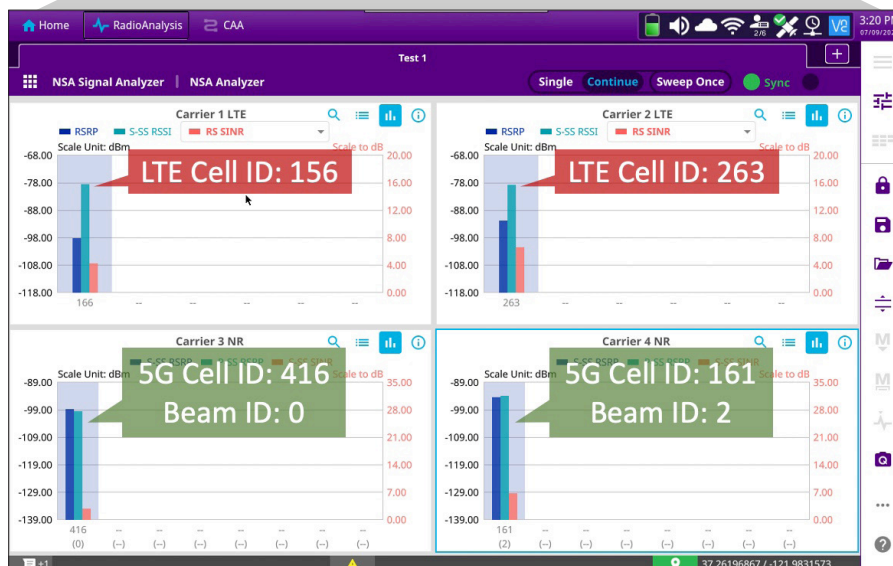
OneAdvisor-800 Non-Stand Alone (LTE and 5G) Signal Analysis
