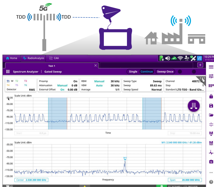
OneAdvisor-800 Dual Gate Spectrum Analysis (TDD Interference)
