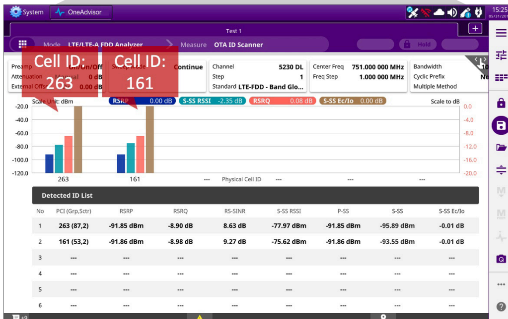
OneAdvisor-800 LTE Signal Analysis
