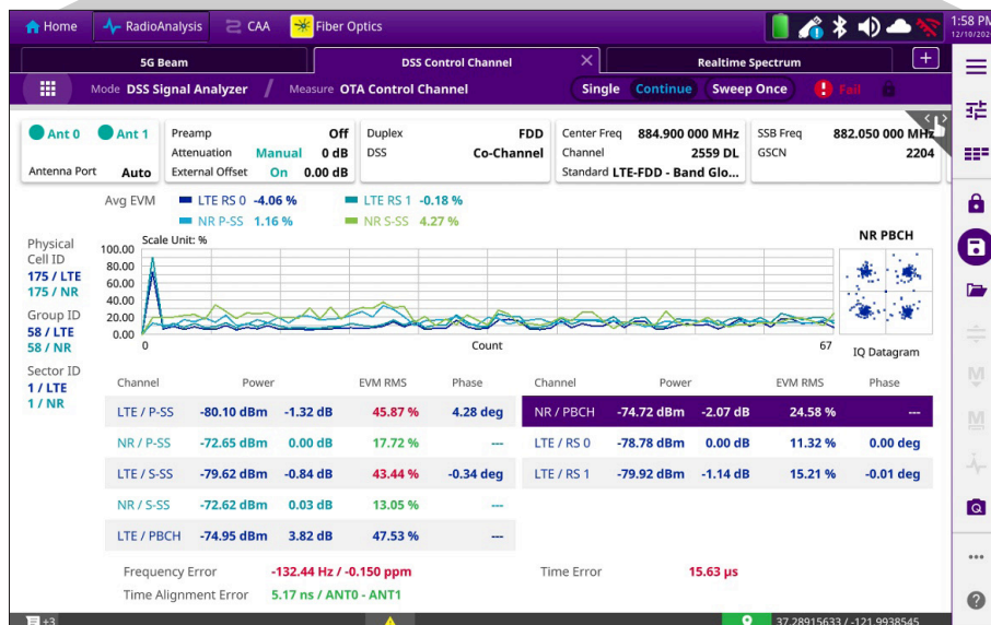
OneAdvisor-800 Dynamic Spectrum Sharing (DSS) Signal Analysis
