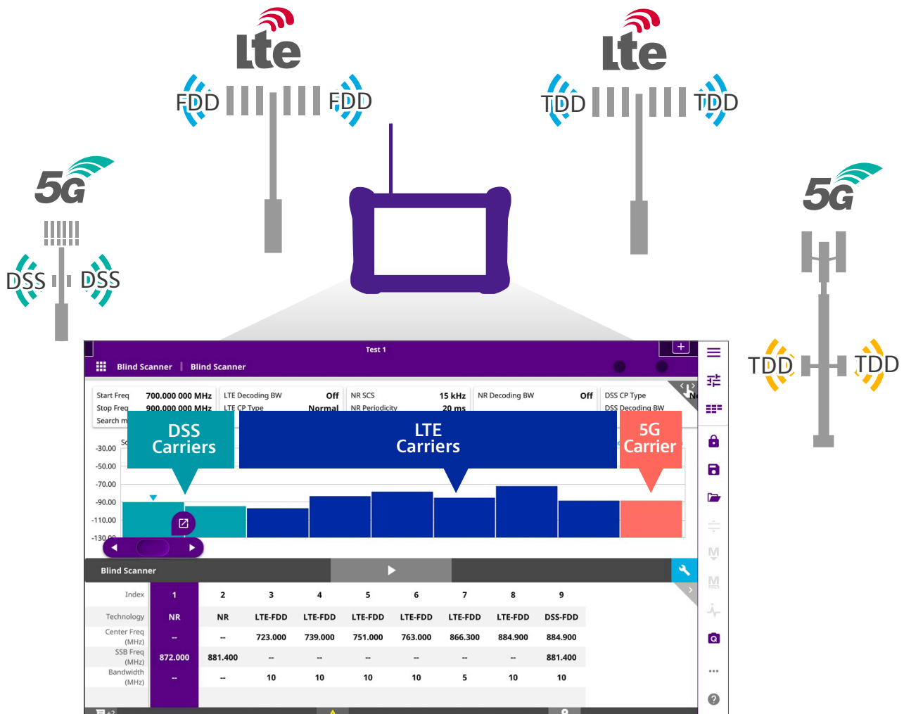
OneAdvisor-800 RF Blind Scanner
